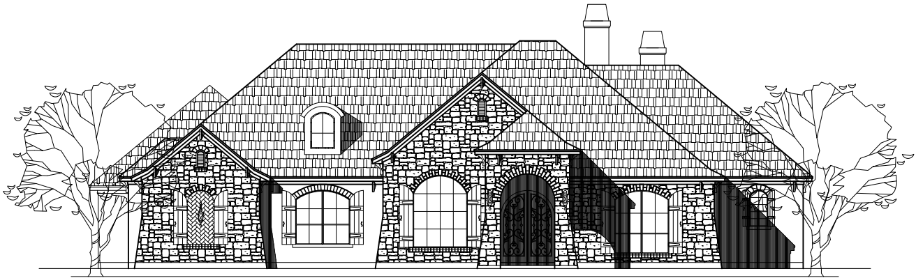
FRONT ELEVATION
